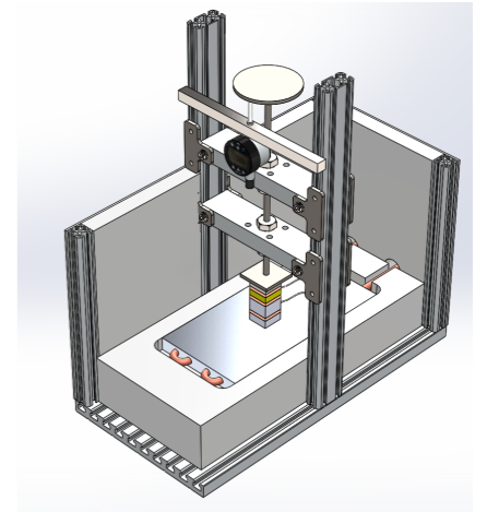
Plate apparatus for determining the thermal conductivity
