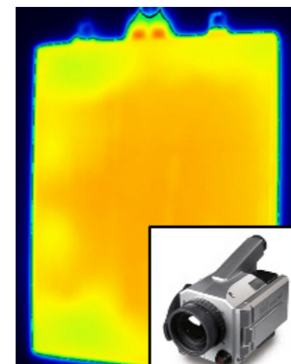
Thermographic image of a lithium-ion pouch cell
