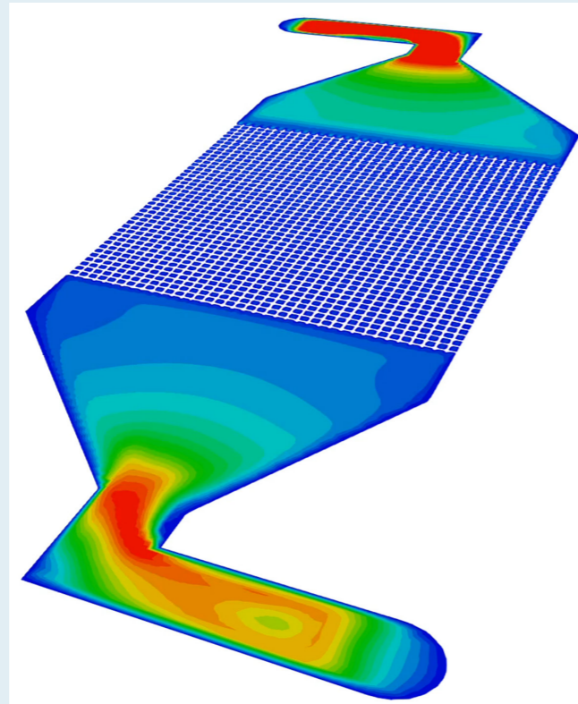
Flow field in an electrolytic cell for electrolysis
