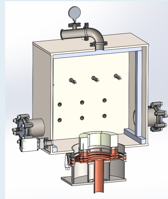
Test rig for thermal characterisation of a thermal interface for space applications
