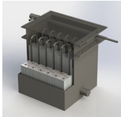
High-performance latent heat thermal energy storage based on a PCM fibre structure composite
