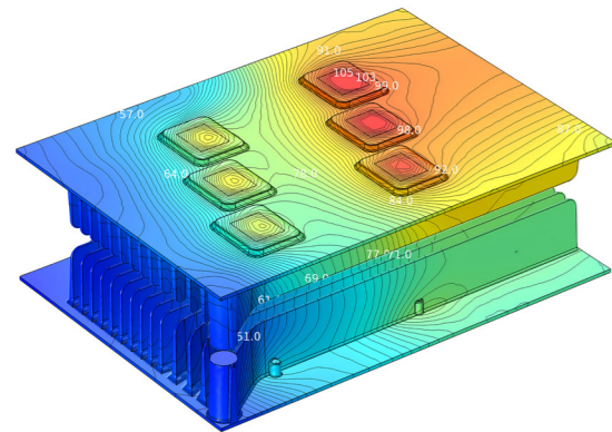
Distribution of the temperature distribution in a heat sink
