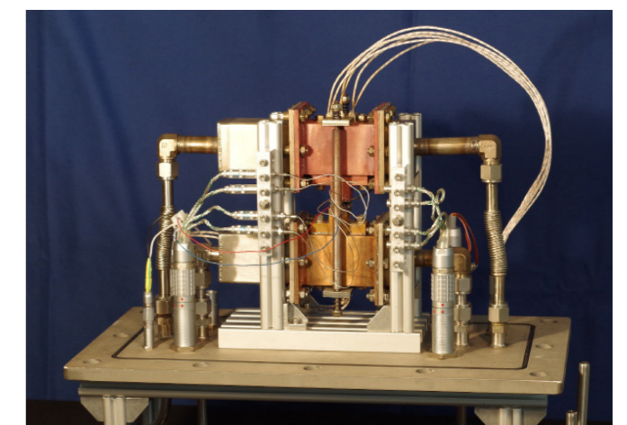
Test rig for characterising thermoelectric modules under cyclic temperature changes
